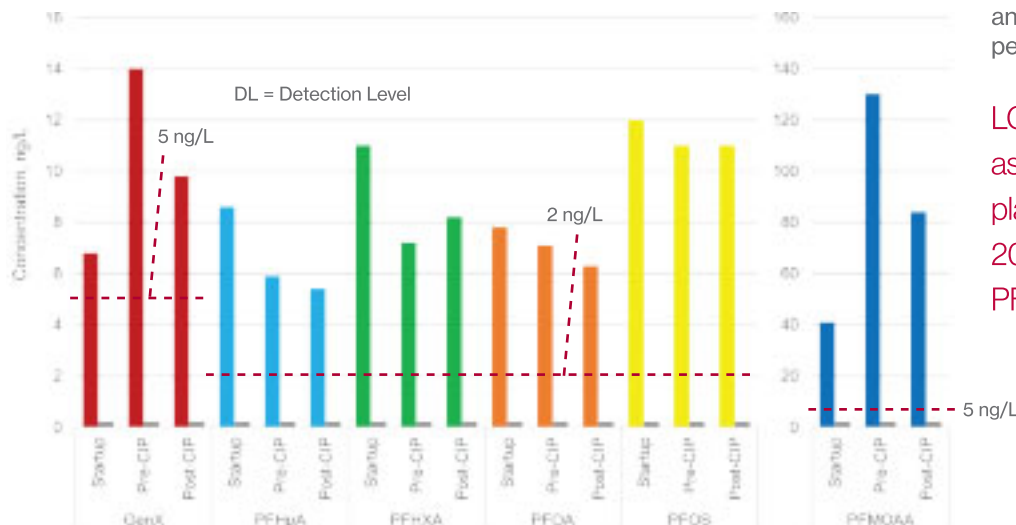
BCNWTP Contaminant Removal via TFN Membrane
